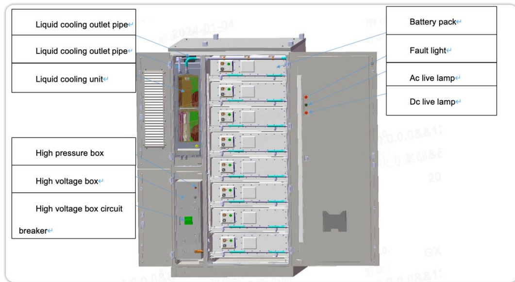
Figure 2.6-2 Cabinet Interior Structure Diagram
