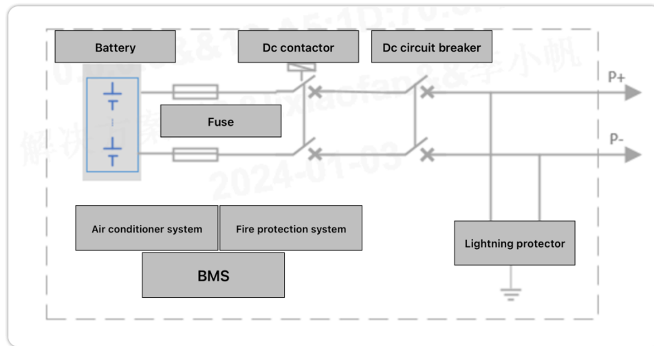
Figure 2.1 Electrical primary diagram
