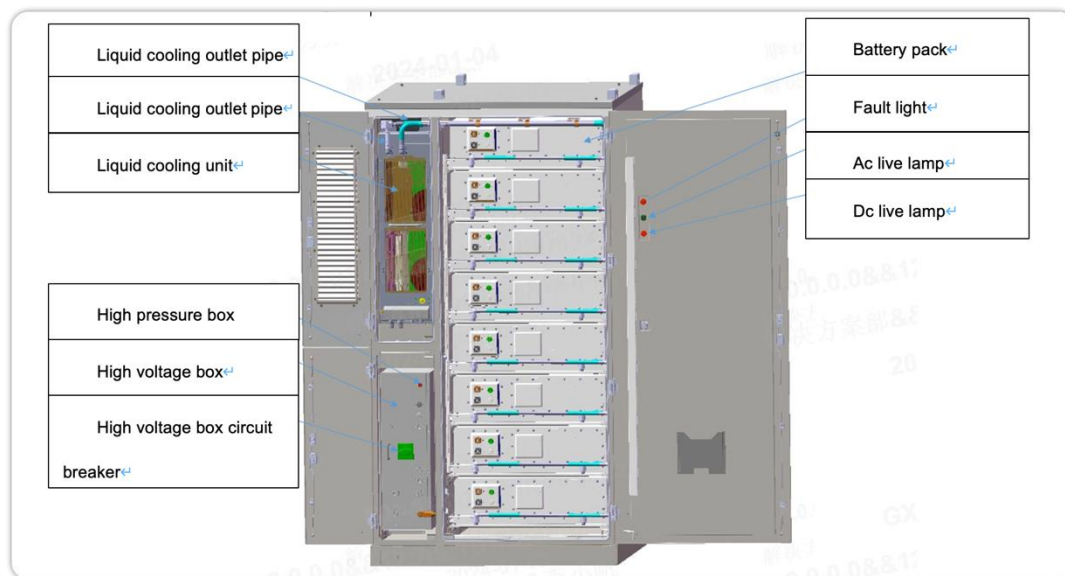
Figure 4.2 Distribution switch location diagram
