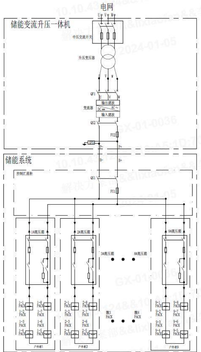
Figure 4.1 Typical architecture diagram for outdoor cabinet use
