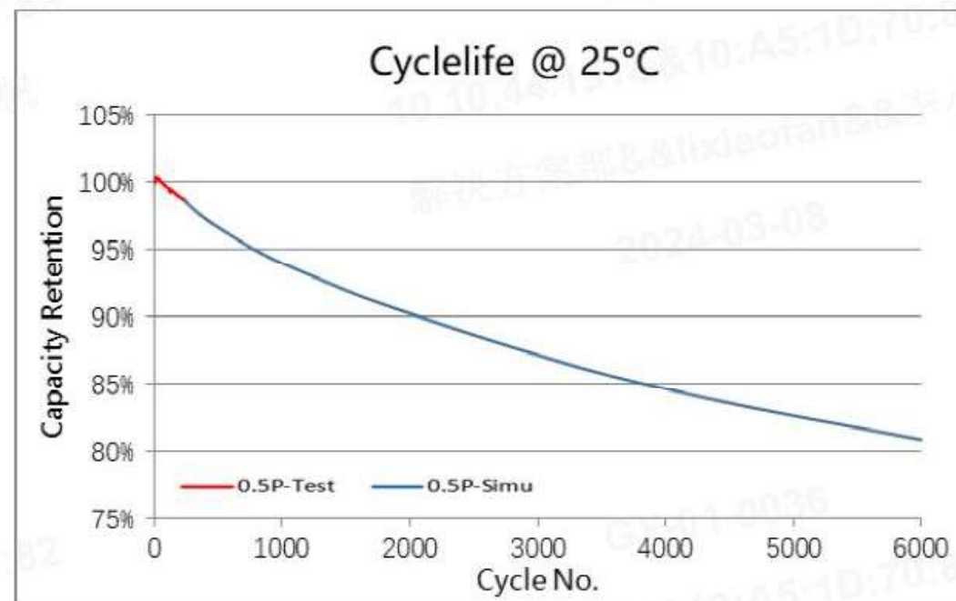
Figure 3.11 Cycle Life 循环寿命
